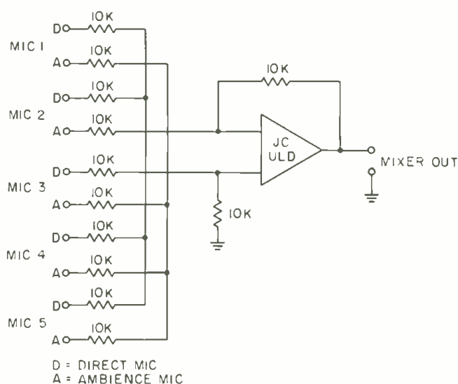
Figure 5. The condenser microphone mixer.
